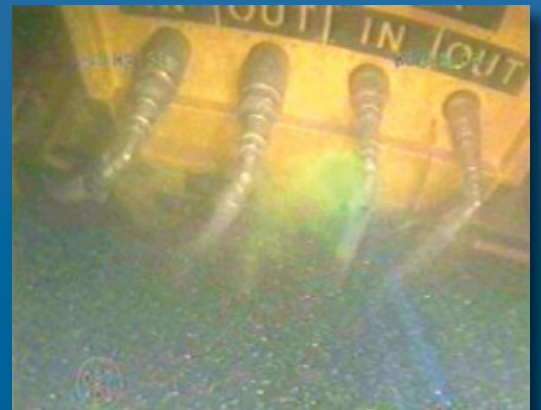
Camera view of excited dye using the Long Ranger Sensor output to graphical display as below The blue excitation light beam is visible Fluoresced light produced by the dye shows as a green cloud at the leak location Tracer dye is Fluorescein
